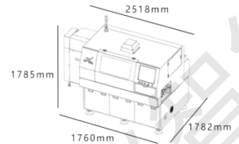
RZS含飞达20站 Includ 20 feeder station
