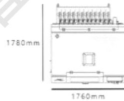
RZS含飞达12站 Including 12 feeder station
